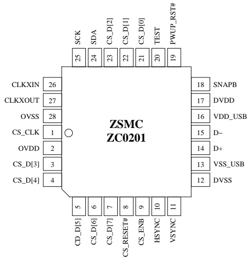
Figure 2 Chip Pin Out Diagram
