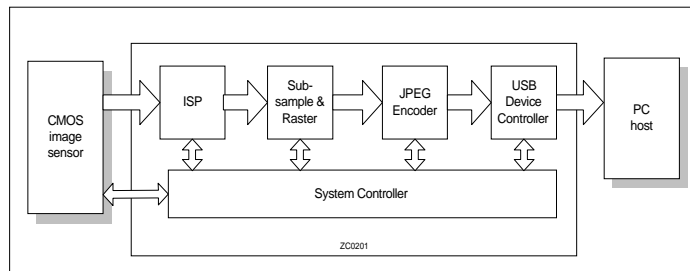
Figure 1 ZC0201 Block Diagram
